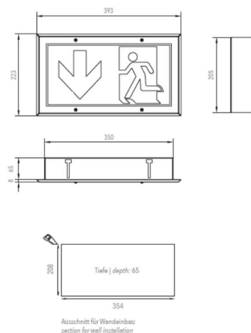
Wandeinbau | wall installation
