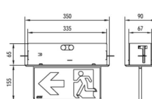
Deckeneinbau (DE) ceiling installation (DE)
