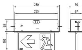
Deckeneinbau (DE) ceiling installation (DE)
